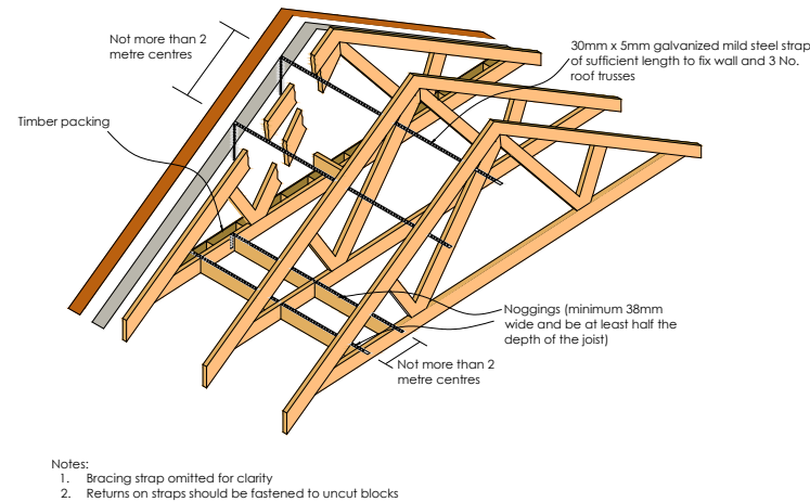
Figure 7: Lateral restraint to gable wall via roof trusses
