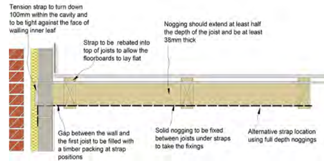
Figure 6: Lateral restraint to floors
