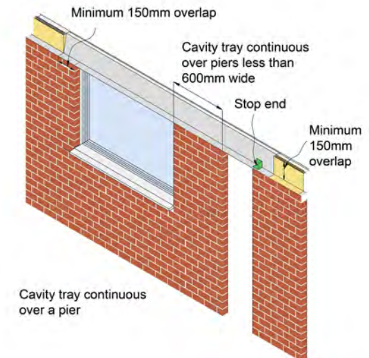
Figure 17: Continuous cavity tray over two openings and a small pier
