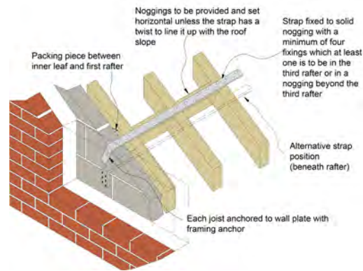
Figure 5: Lateral restraint strap to gable wall
