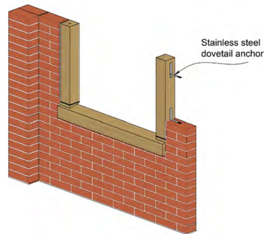
Figure 25: Stone jamb and mullion, fixing to walls
