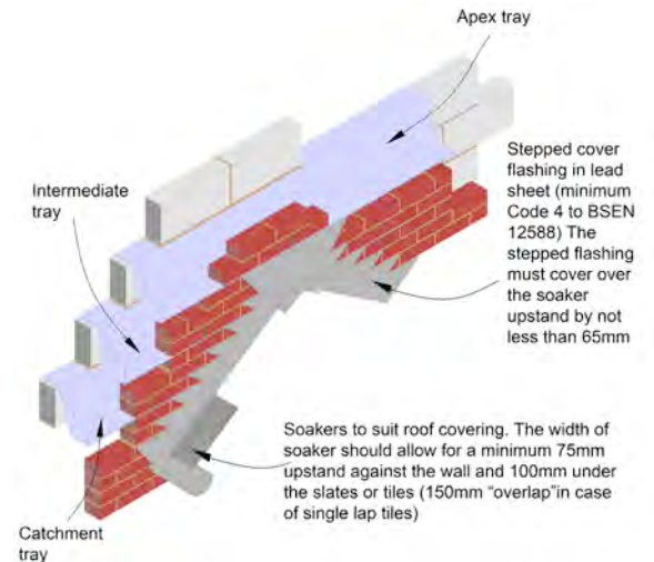
Figure 20: Stepped cavity at roof/wall abutments
