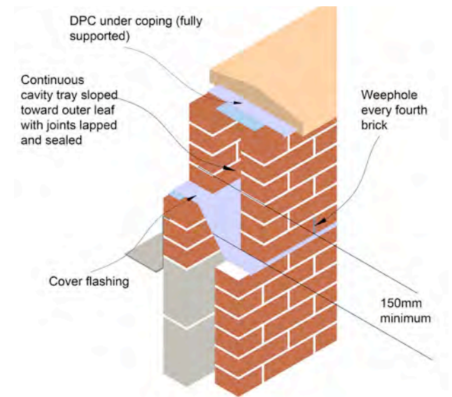
Figure 21: Parapet wall detail
