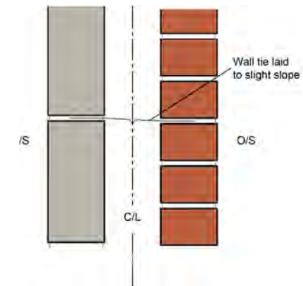
Figure 8: Wall tie provision
