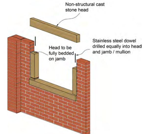
Figure 26: Joining stone jambs to sills and head
