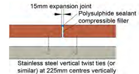
Figure 13: Typical expansion joint detail
