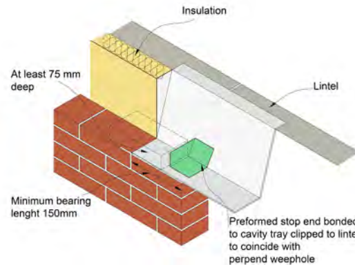
Figure 18: Stop-end to cavity tray
