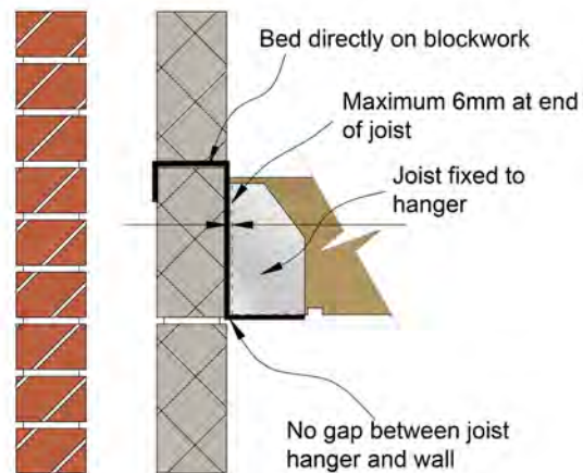
Figure 3: Typical restraint type joist hanger
