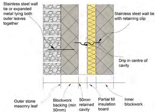
Figure 24: Masonry cavity wall with stone outer leaf
