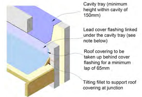
Figure 16: Cavity tray over a flat roof/wall abutment
