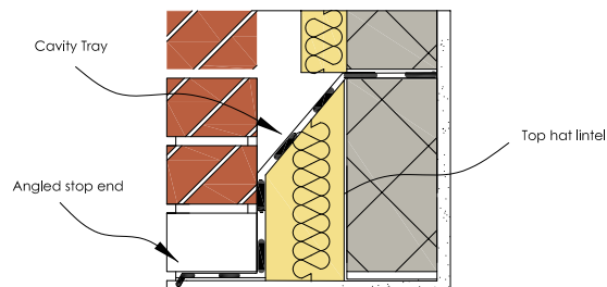
Figure 19: Stop-end in relation to cavity tray and lintel
