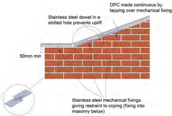
Figure 23: Fixing of copings to sloping parapets
