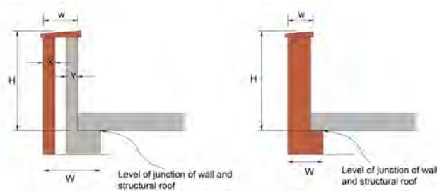
Figure 22: Maximum height of parapet walls (to be read in conjunction with Table 4)
