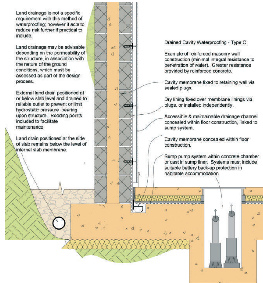
Figure 4: Type C drained protection
