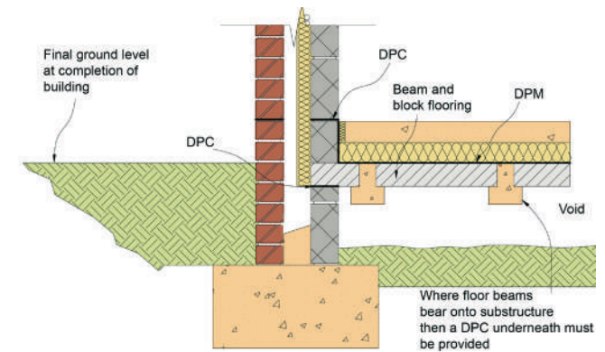
Figure 14: Typical pre-cast beam and block floor with DPM
