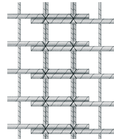
Figure 12: Typical reinforcing lap
