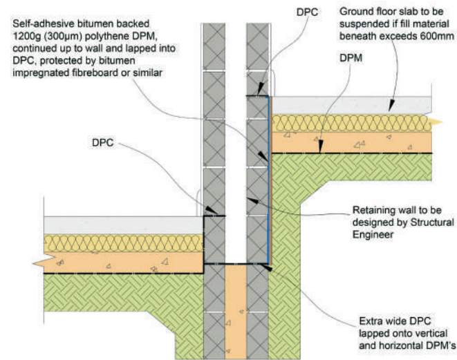
Figure 8: Stepped damp proof membrane
