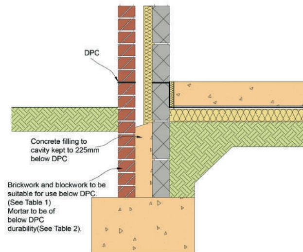
Figure 6: Concrete cavity fill- traditional ground bearing slab
