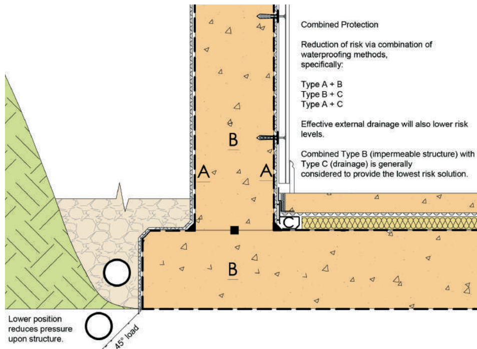
Figure 5: Combined protection
