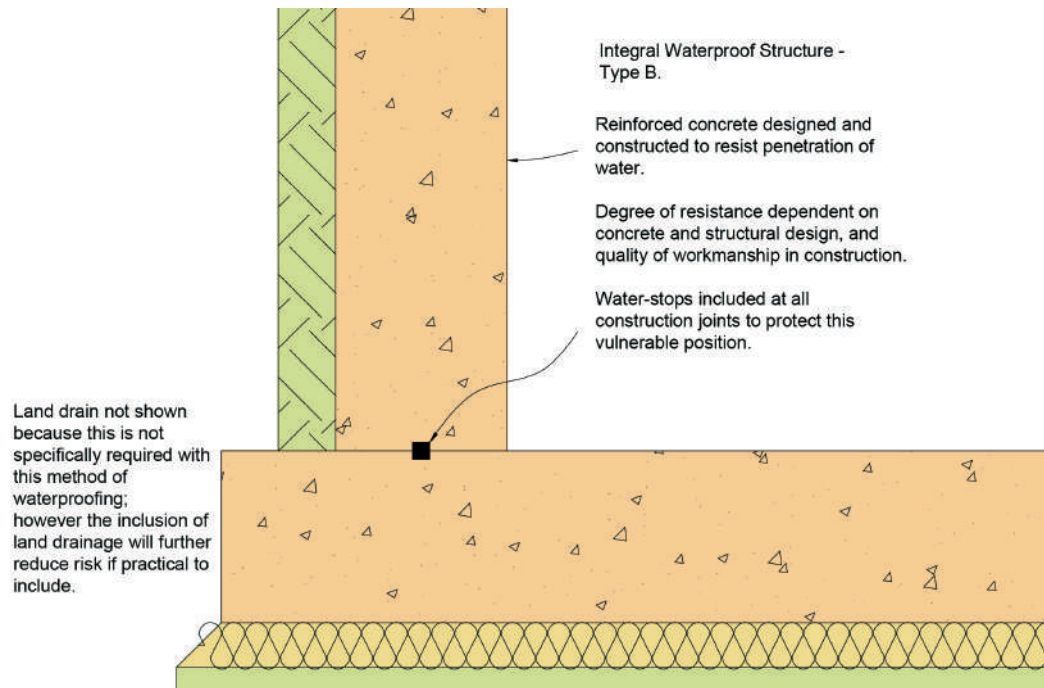
Figure 3: Type B Structurally integral protection
