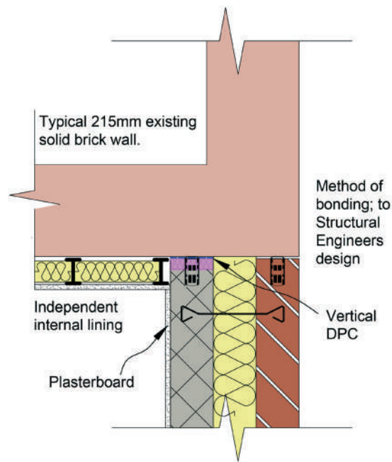
Figure 8 - Bonding new walls to existing solid masonry wall
