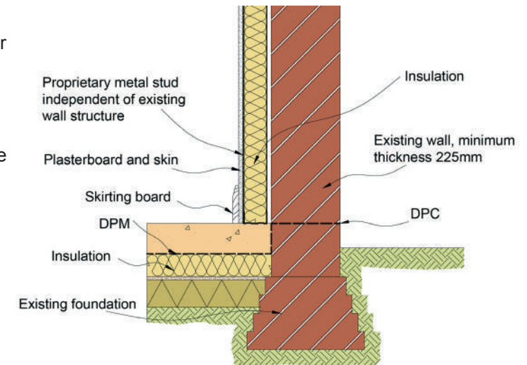
Figure 6: Typical independent internal lining
