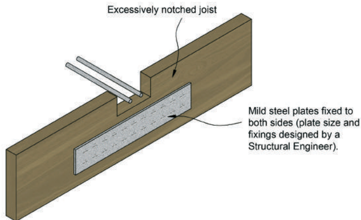
Figure 5: Strengthening excessively notched joist
