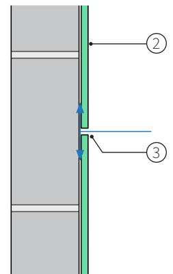
Partially bonded
